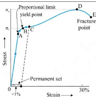
Fig. 8.2 A typical stress-strain curve for a metal.
